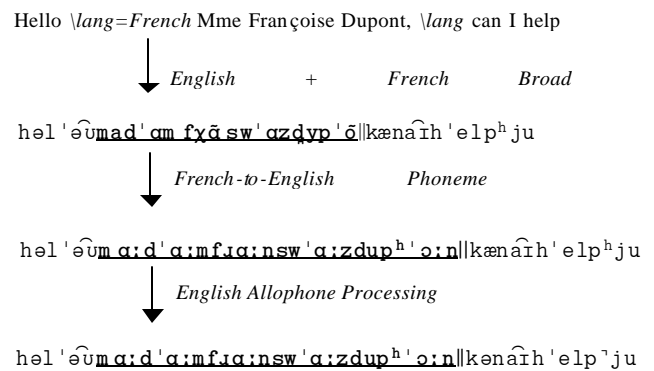
Figure 2. Phonetic transcription of a mixed-language text
