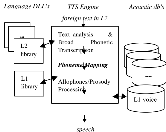
Figure 1. Foreign pronunciation flow in the TTS architecture
